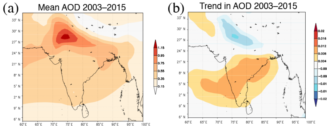
Figure 7. (a) Mean May–June aerosol optical depth at 550 nm (AOD550) in the MACC reanalysis for 2003–2015. (b) Trend in AOD550 over this period ( \text{yr}^{-1} ).
