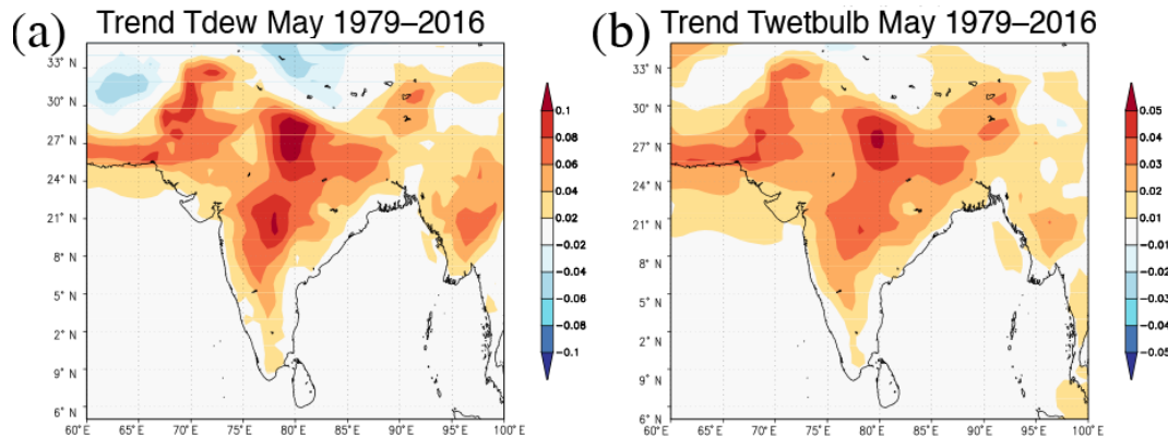
Figure 8. Trend in (a) dew point temperature, (b) wet bulb temperature in ERA-Interim over May ( \text{K yr}^{-1} ).
