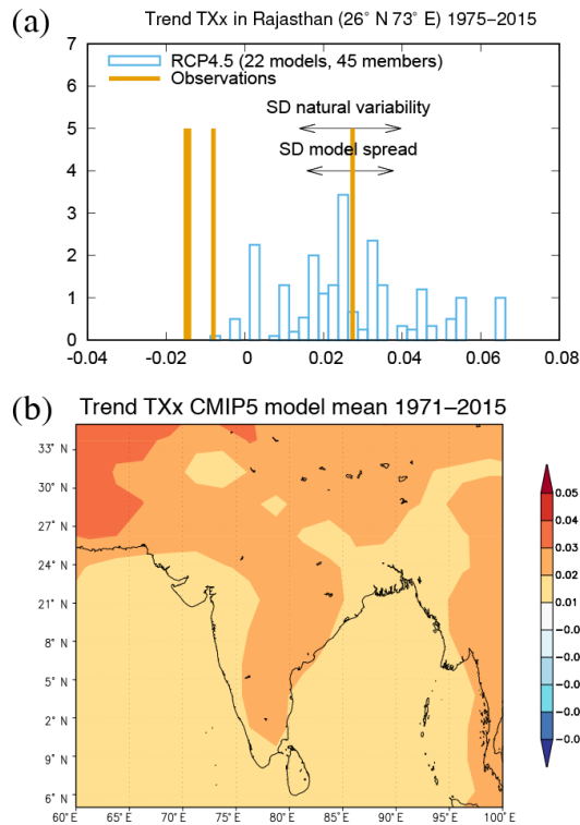
Figure 10. (a) Histogram of the trend in TXx ( \text{K yr}^{-1} ) at the grid point closest to 26^\circ \text{N} , 73^\circ \text{E} in the CMIP5 ensemble (excluding the MIROC models). Ensemble members of the same model are down-weighted so that each model gets a weight of 1. This is compared with observations: the trends in Bikaner (corrected for varying missing data), Jodhpur and the nearest grid point of the ERA-Interim reanalysis (left three bars). For reference the trend in the IMD gridded dataset without correction for varying missing data is also given (rightmost bar). (b) Mean of trend in TXx ( \text{K yr}^{-1} ) in the CMIP5 ensemble 1971–2015, with historical experiments up to 2005 extended with the RCP4.5 2006–2016 simulations.
