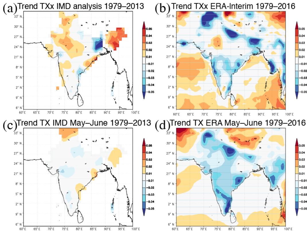
Figure 4. (a) Trend in the highest maximum temperature in the IMD gridded daily analysis for 1979–2013 ( \text{K yr}^{-1} ). (b) Same as in the ERA-Interim reanalysis for 1979–2016. (c, d) Same as (a, b) but for the mean May–June maximum temperature trends.
