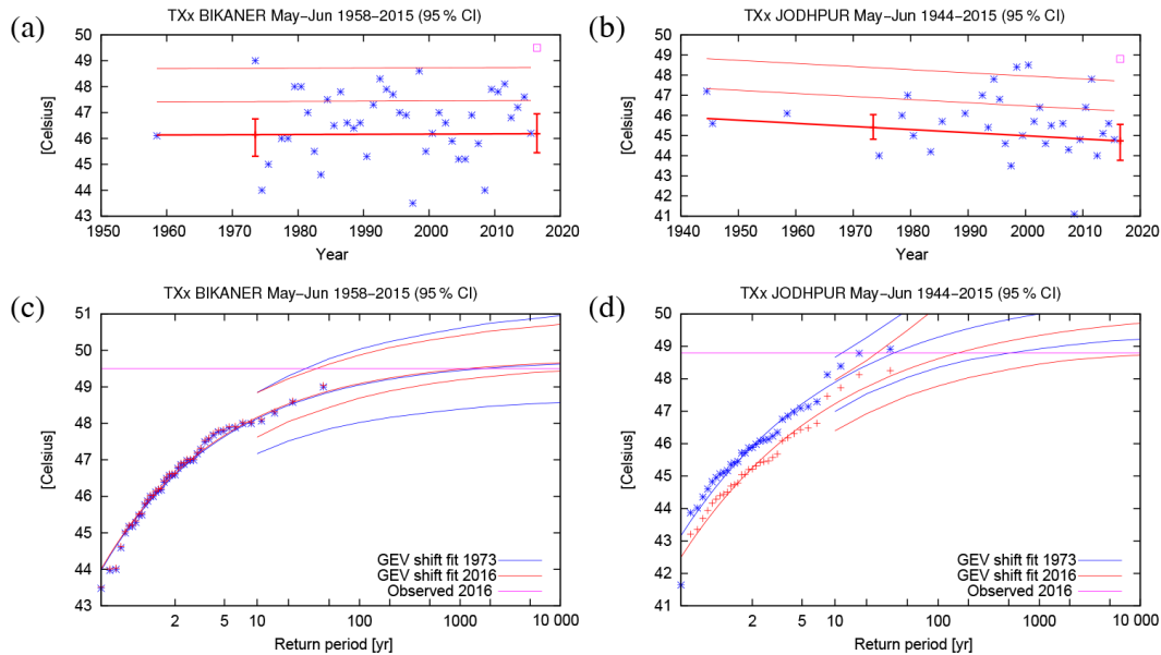
Figure 6. (a) Observed TXx at Bikaner, Rajasthan, India (GHCN-D v3.22) with a GEV that shifts with time fitted (excluding 2016), demanding 70 % valid data in May–June. The thick line denotes \mu and the thin lines \mu + \sigma and \mu + 2\sigma . (b) Same for Jodhpur. (c) Gumbel plot of the fit in 1973 and in 2016 (central lines). The upper and lower lines denote the 95 % confidence interval. The observations are shown twice, shifted up and down with the fitted trend. (d) Same for Jodhpur.
