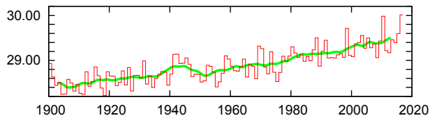
Figure 3. March–May mean sea surface temperature in the northern Indian Ocean (EQ 30° N, 60–100° E) (°C). Source: ERSST v4 (Huang et al., 2015).
