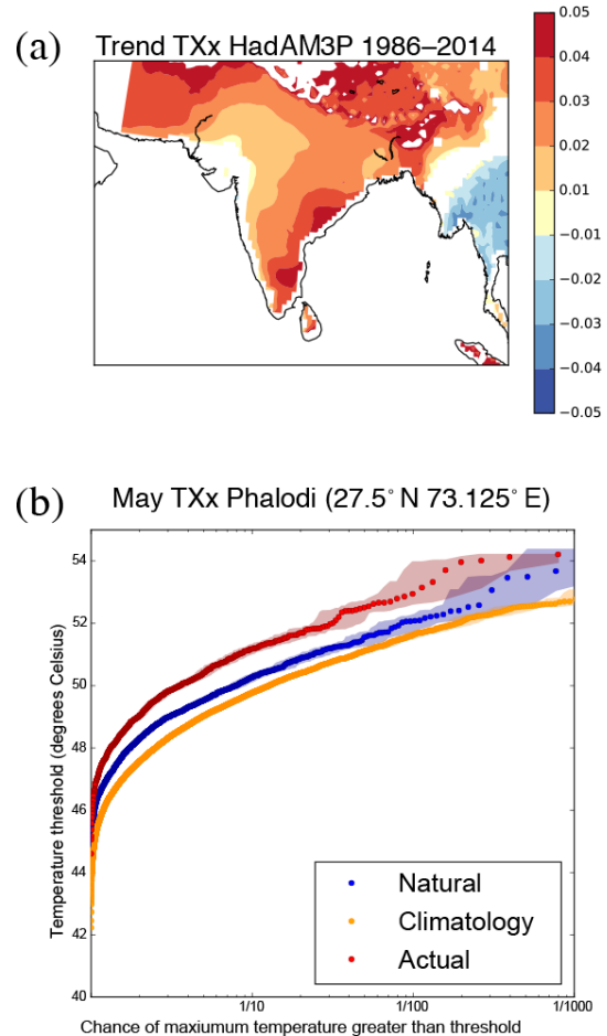
Figure 11. (a) HadAM3P model trend for 1986–2014 of TXx in May ( \text{K yr}^{-1} ). Ocean points and areas not significant at p < 0.05 are shown as white. (b) Return time plots for TXx in May at the grid box closest to Phalodi for “actual” 2016 simulations (red), “natural” 2016 simulations (blue) and Climatology 1986–2014 simulations (yellow).
