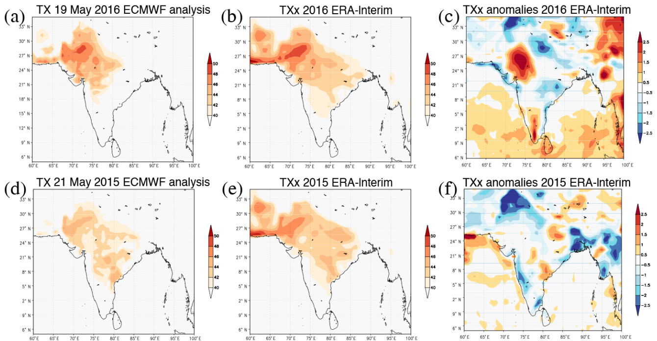
Figure 1. (a) ECMWF operational analysis of the daily maximum temperature on 19 May 2016 ( ^{\circ}\text{C} ); (b) ERA-Interim highest maximum temperature of the year, TXx, in 2016 ( ^{\circ}\text{C} ); (c) anomalies of TXx in 2016 relative to 1981–2010 (K). (d–f) Same as (a–c) but for 21 May 2015, showing the heat wave in Andhra Pradesh and Telangana in 2015.
