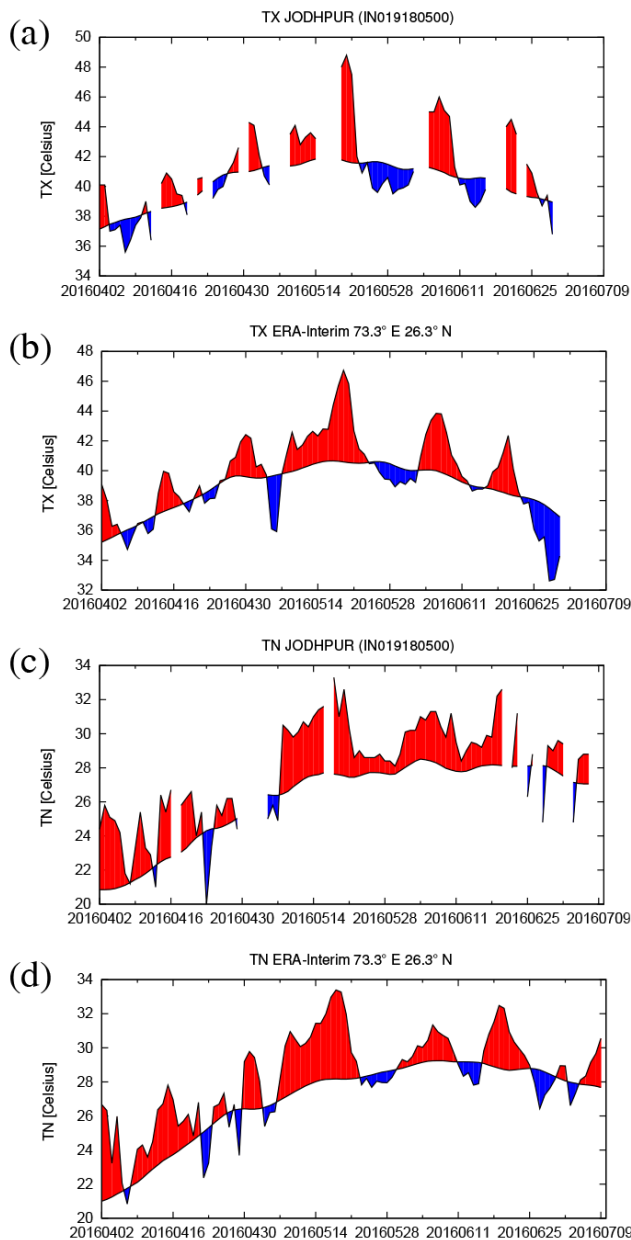
Figure 5. April–June daily maximum temperature time series from (a) GHCN-D v3.22 observations at Jodhpur, the closest station to Phalodi with publicly available data; and (b) ERA-Interim interpolated at the coordinates of Jodhpur ( ^{\circ}\text{C} ). (c, d) Same for the daily minimum temperature. Departures from each dataset’s climatology (1981–2010) are shown in red (positive) and blue (negative). Days with missing data are left white.
